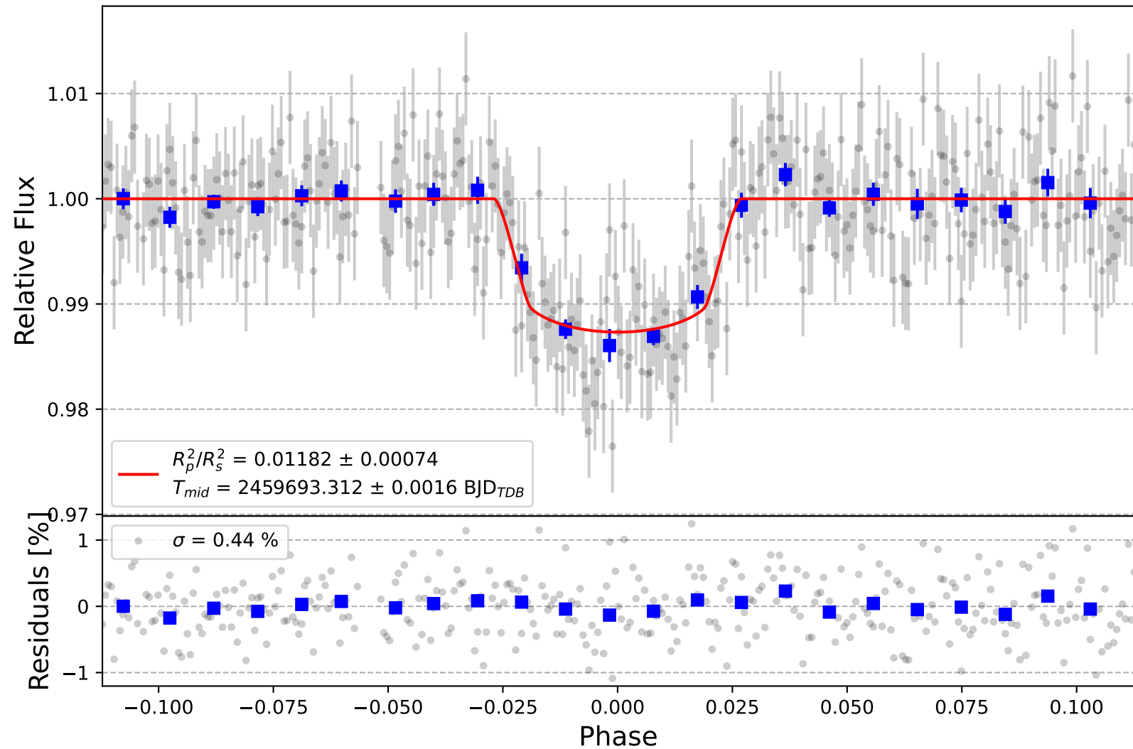
WASP-92 b
