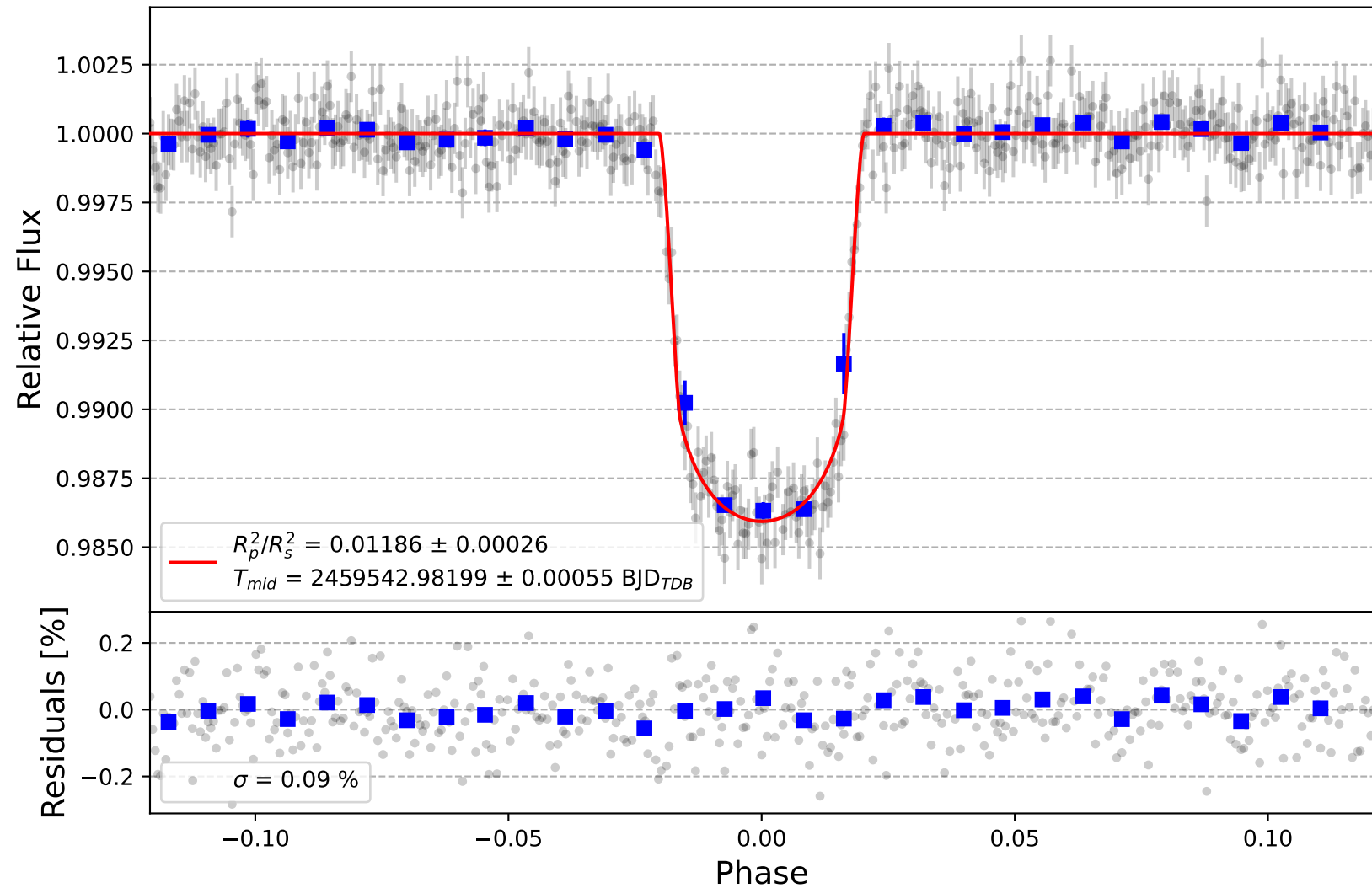
WASP-85 A b
