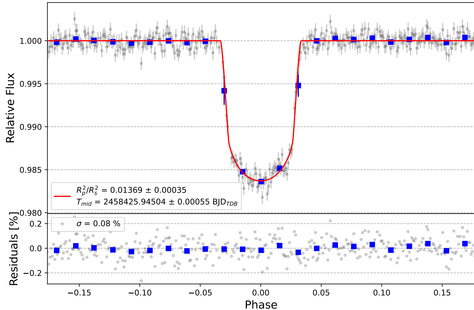
WASP-77 A b
