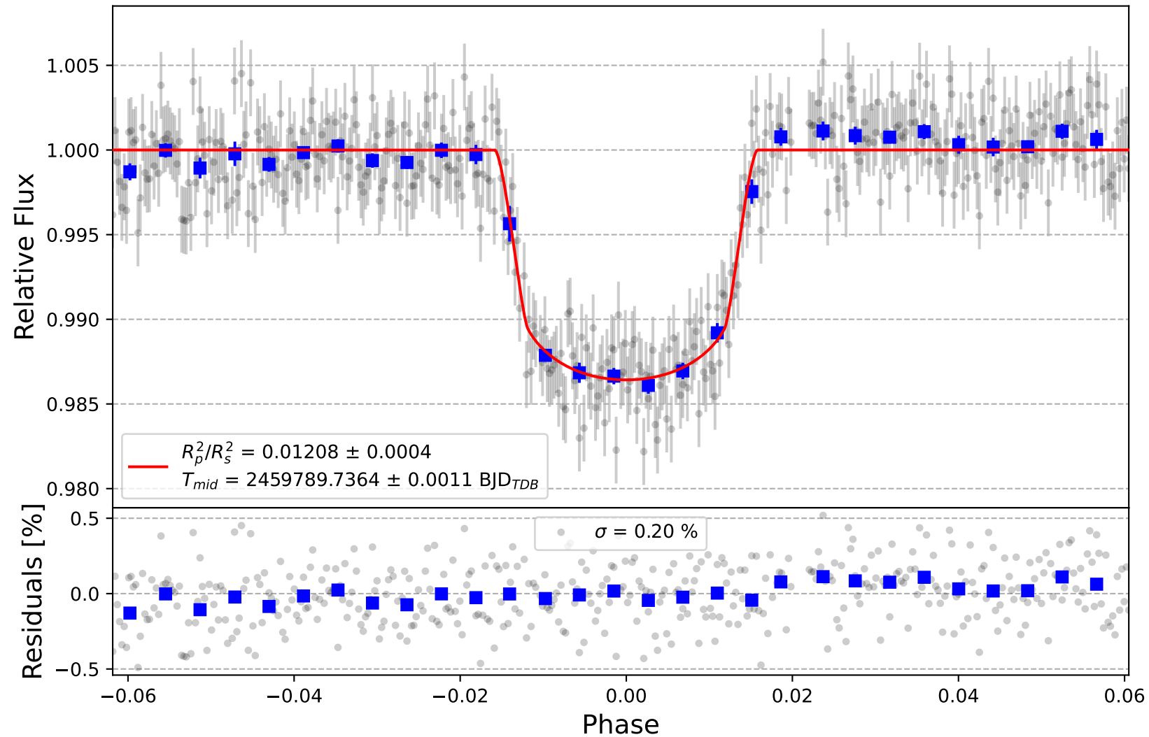
WASP-58 b
