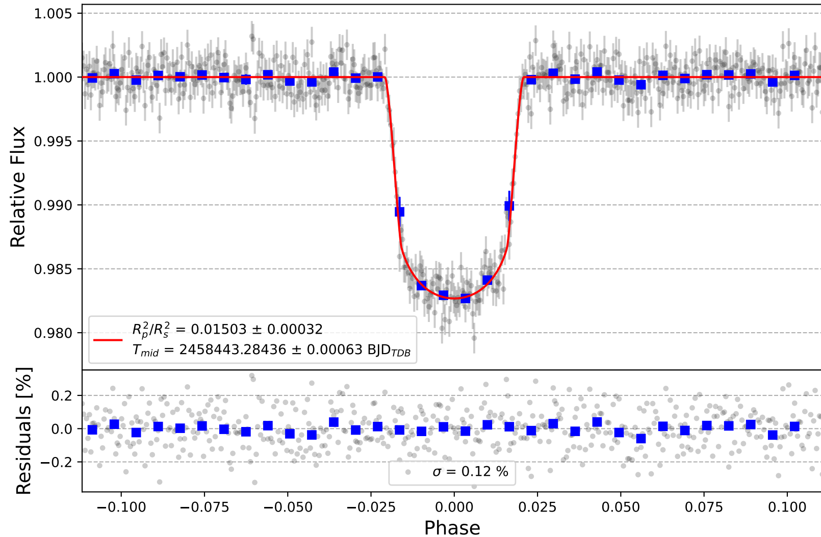
WASP-35 b
