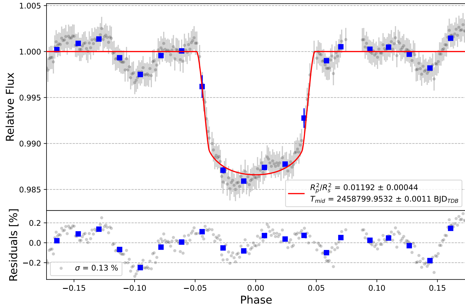
WASP-33 b
