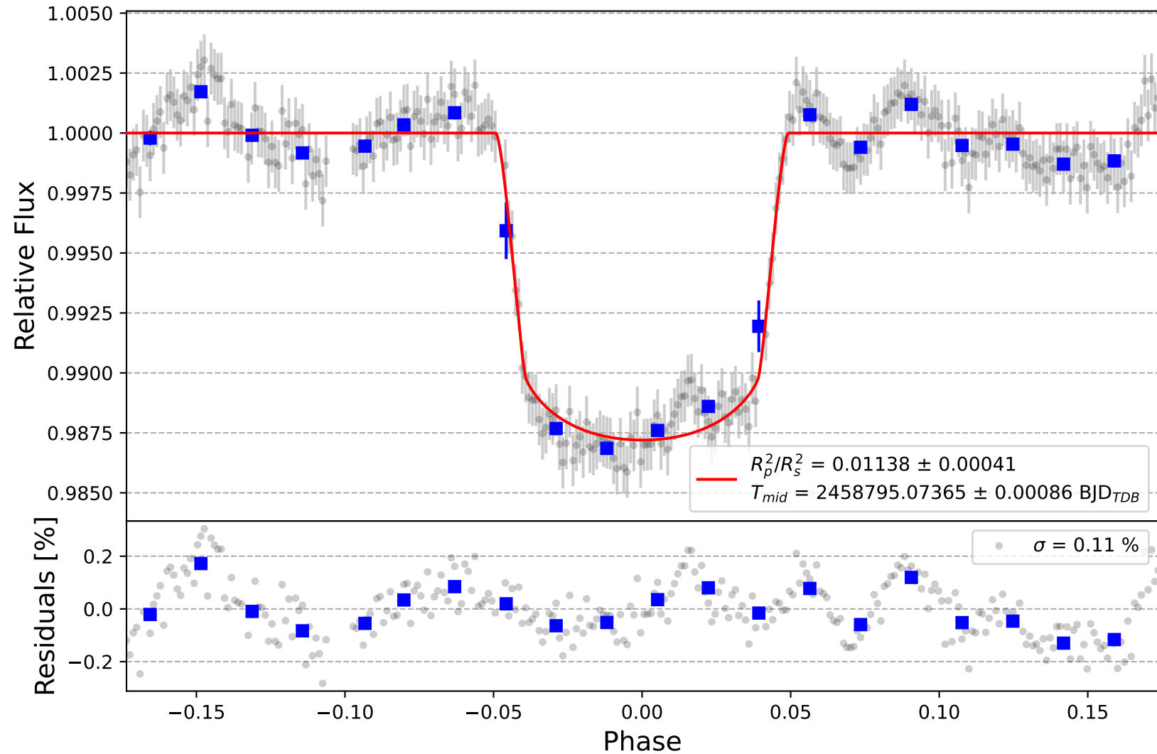
WASP-33 b
