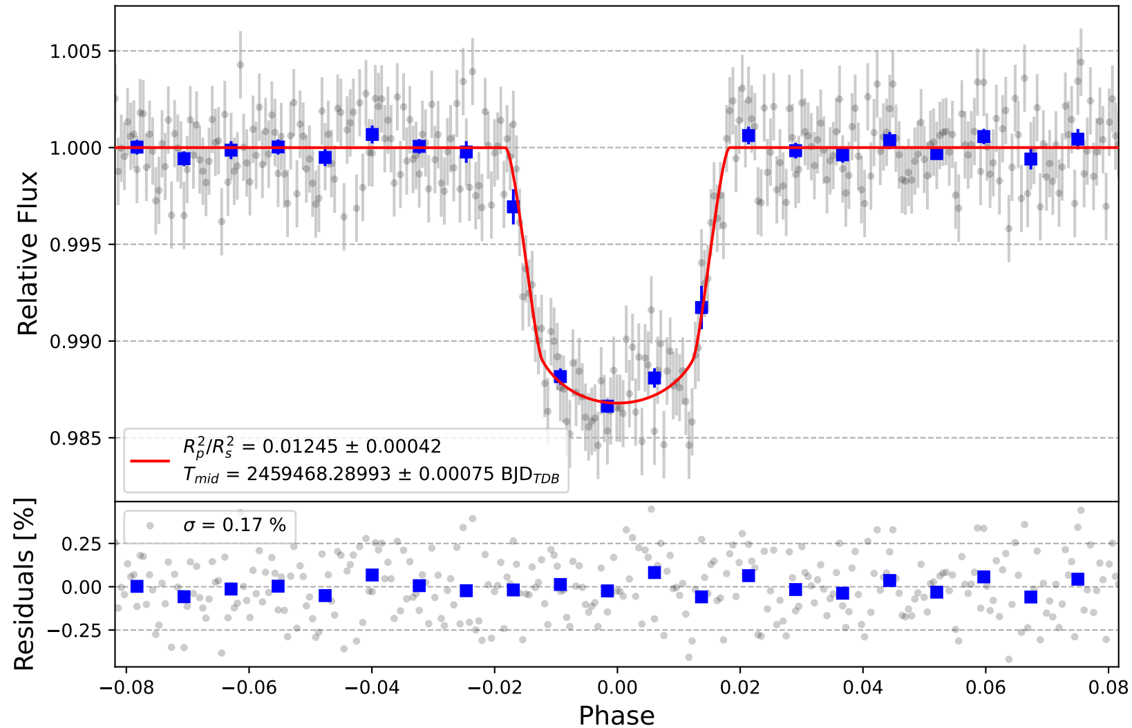
WASP-32 b
