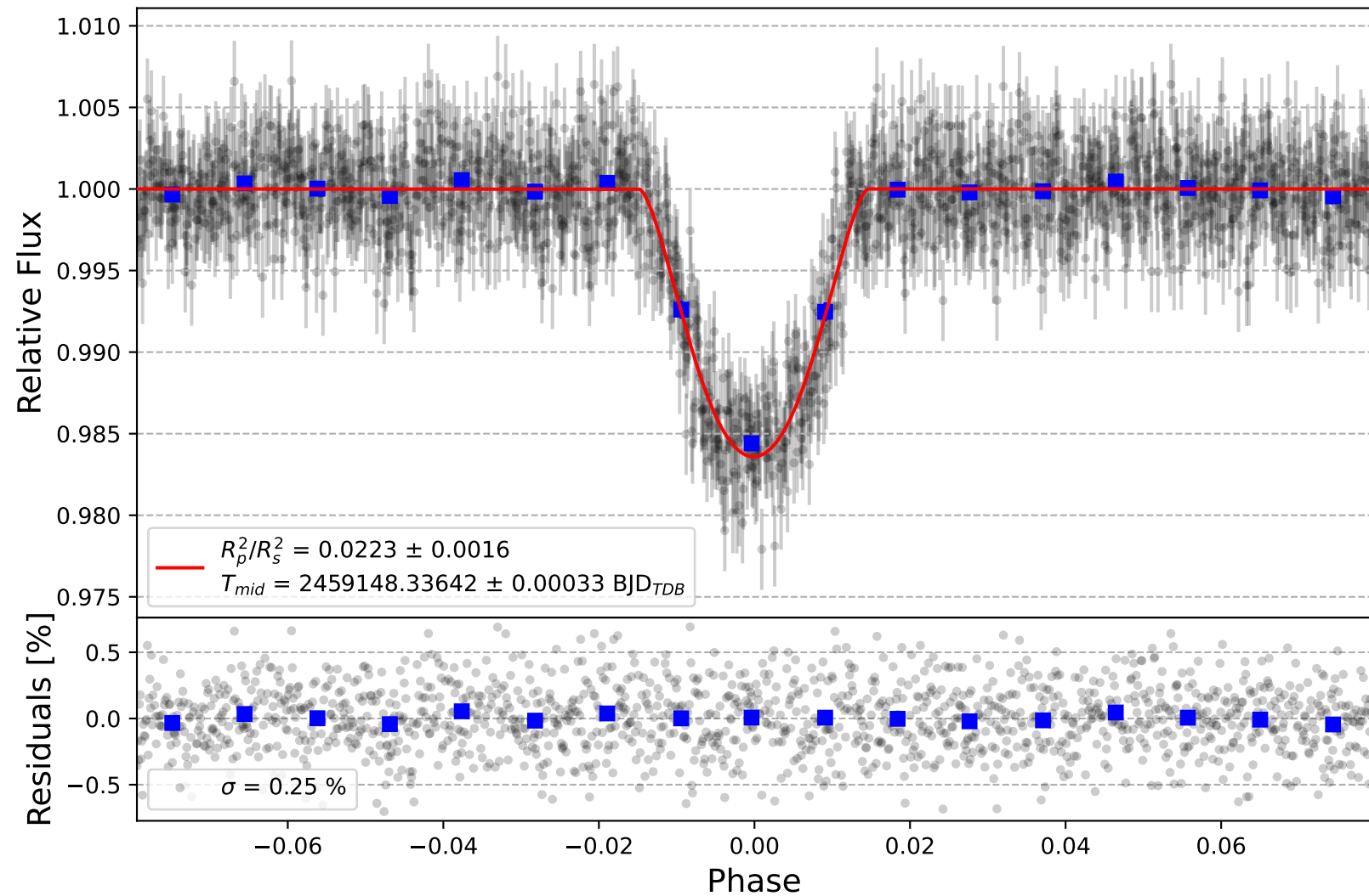
WASP-140 b
