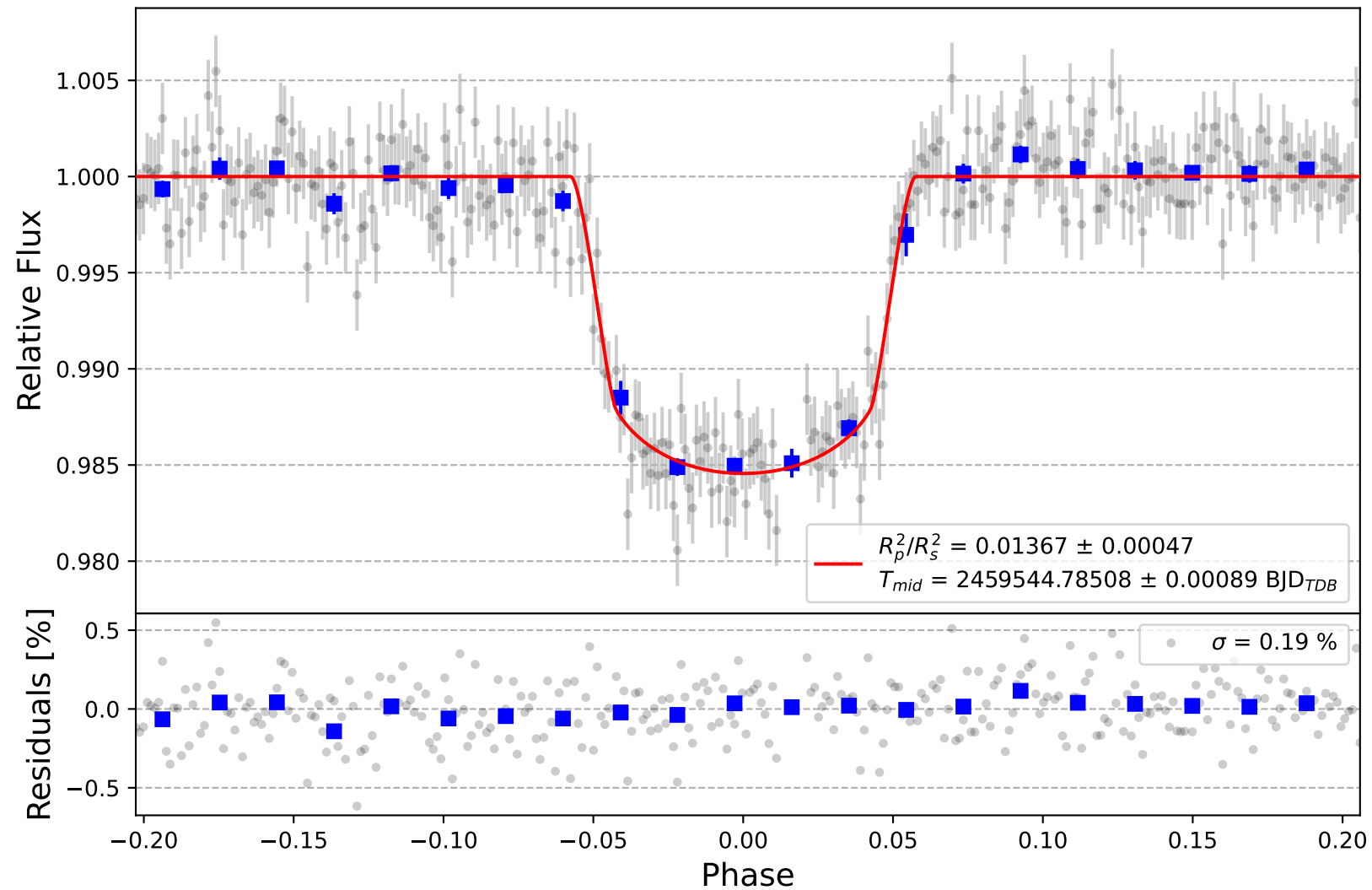
WASP-12 b
