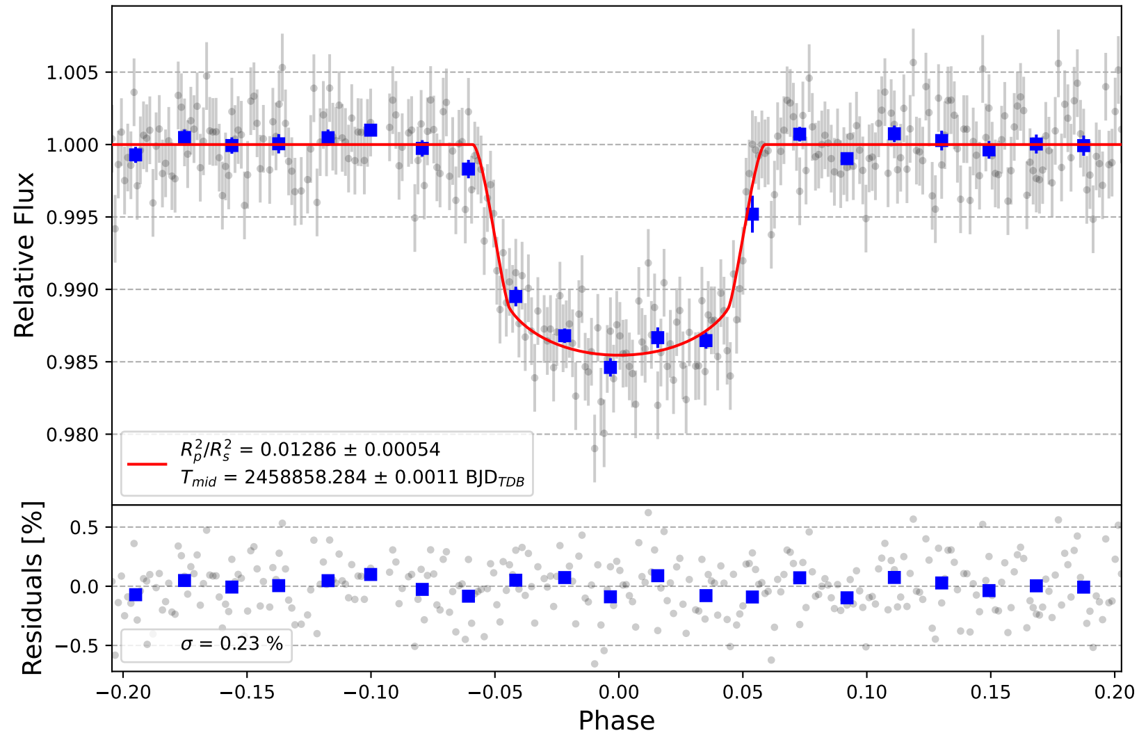
WASP-12 b
