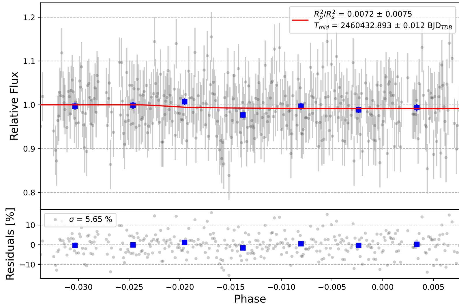
TIC 257060897 b
