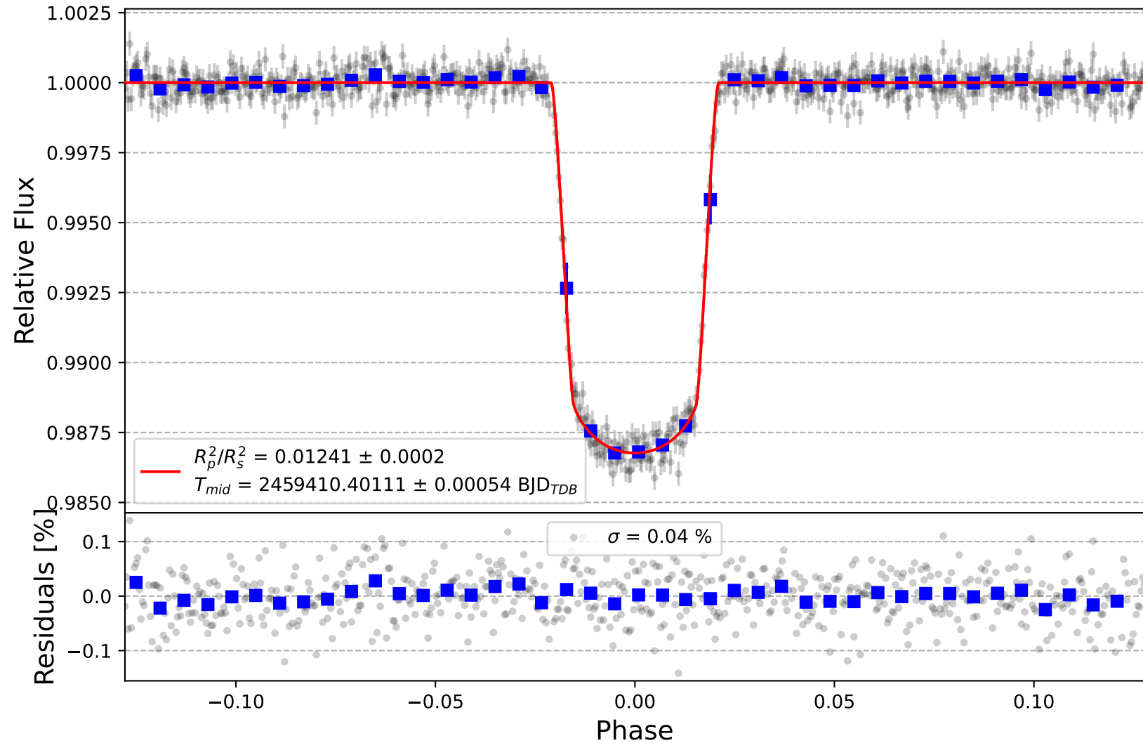
KELT-20 b
