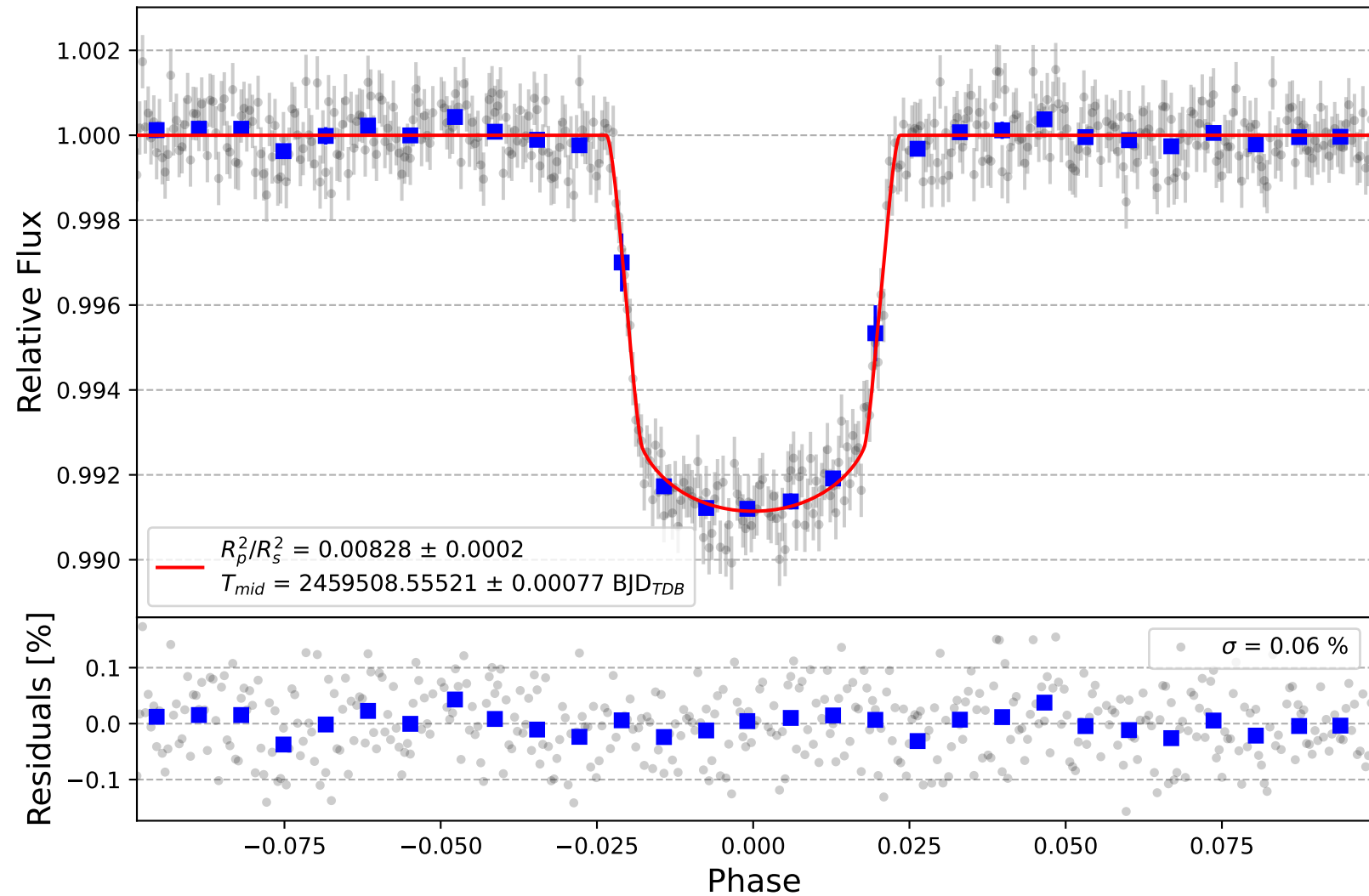
KELT-17 b
