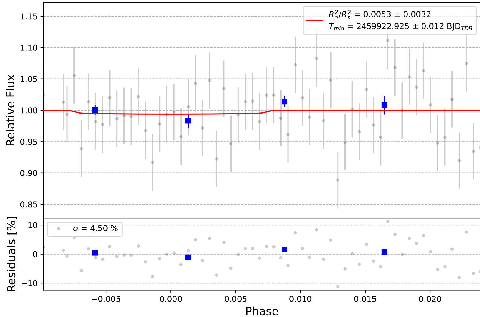
K2-343 b
