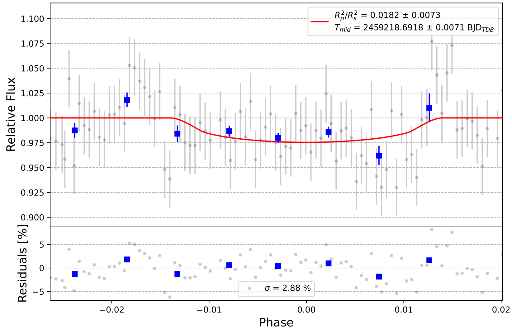
K2-295 b
