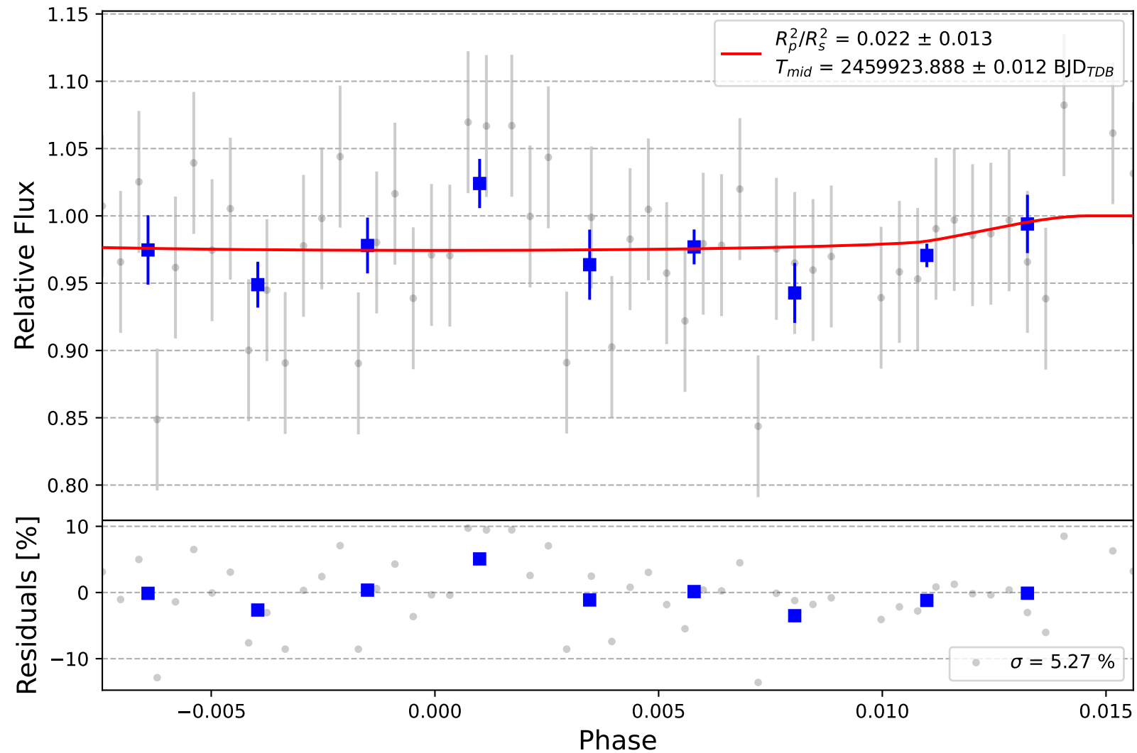
K2-271 b
