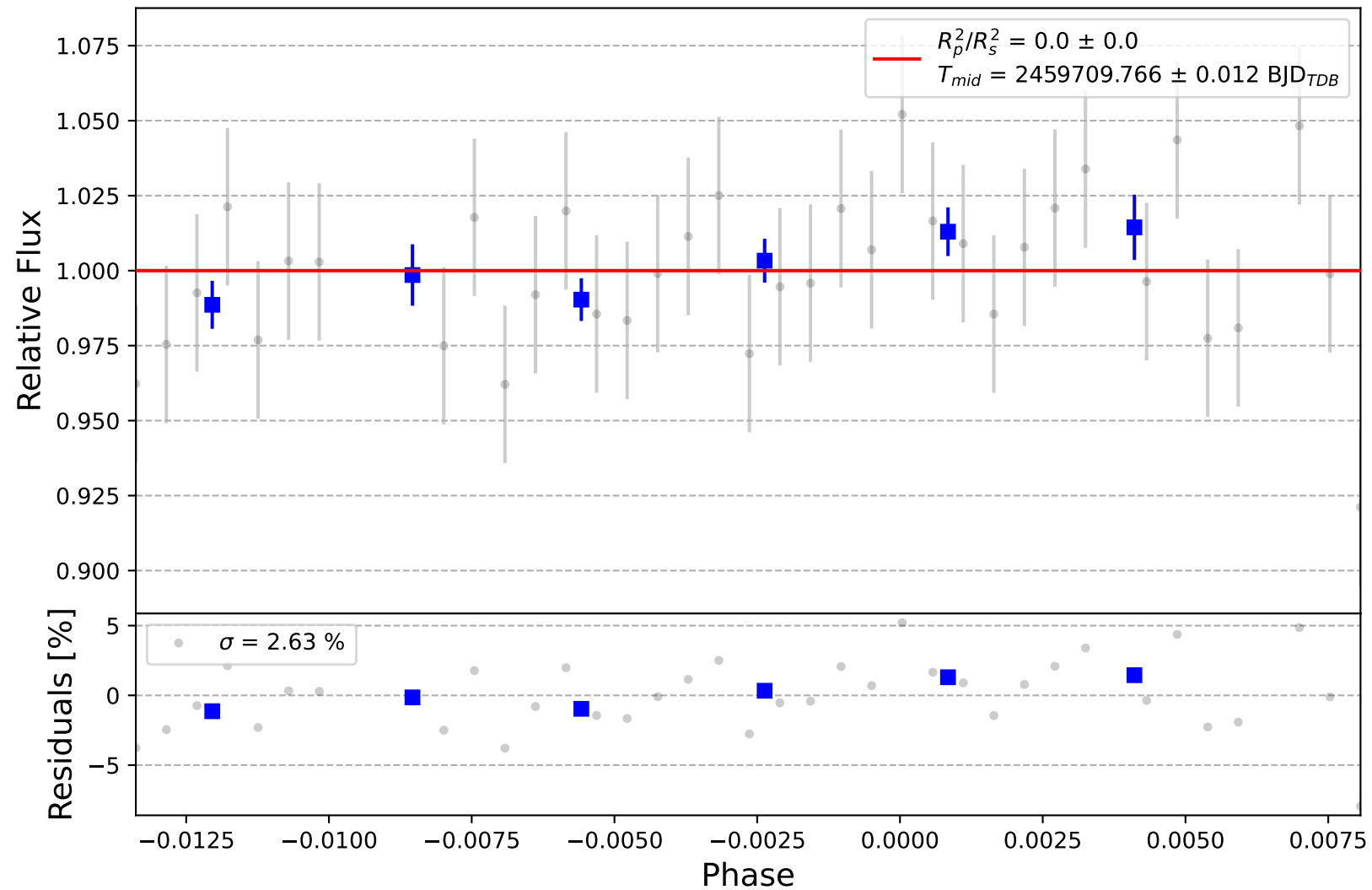
K2-242 b
