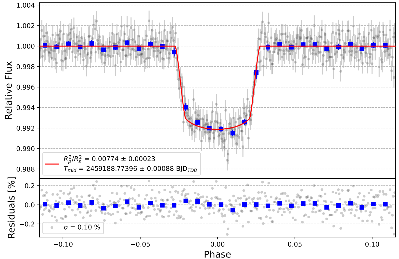
HAT-P-70 b
