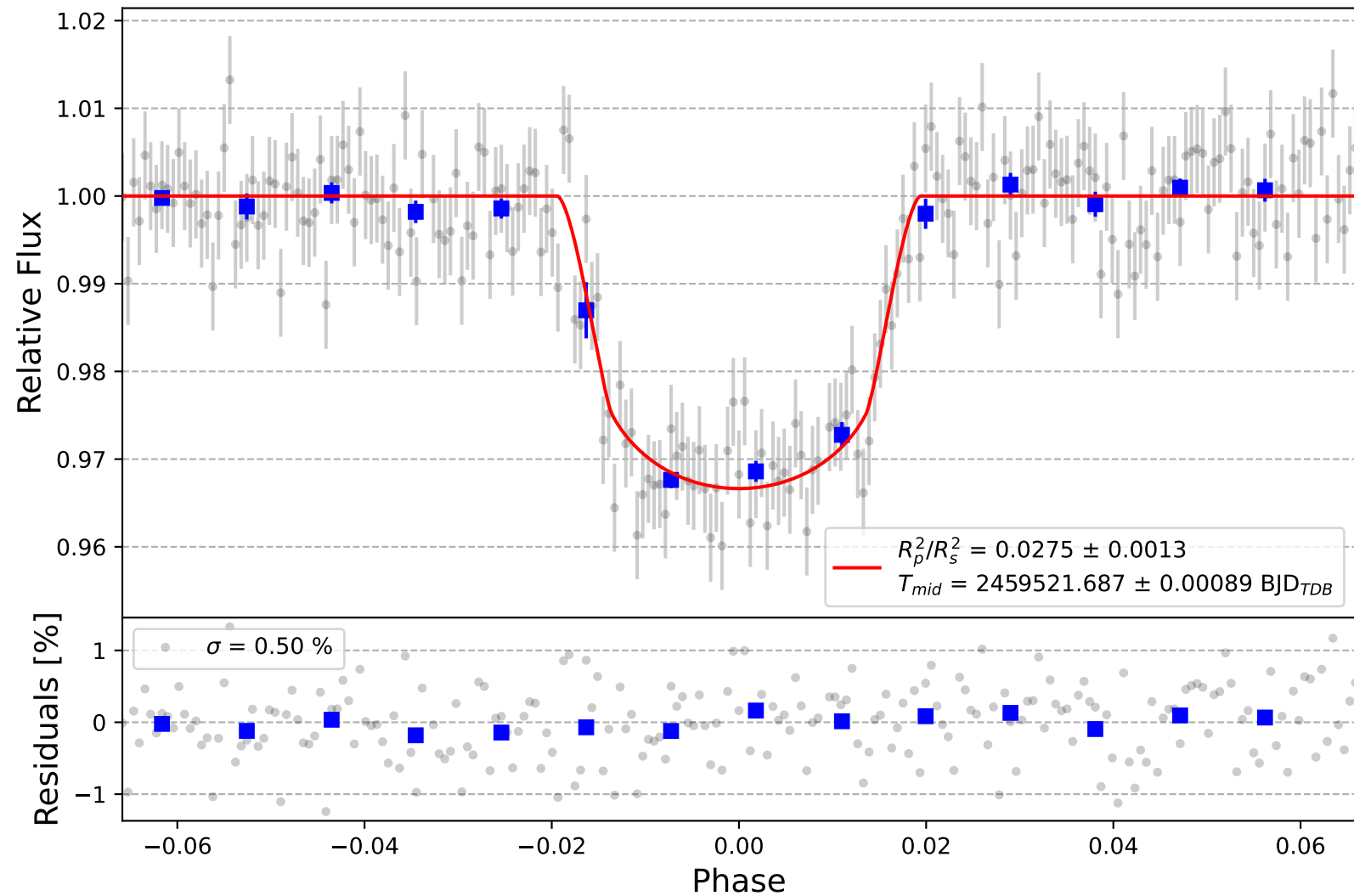
HAT-P-68 b
