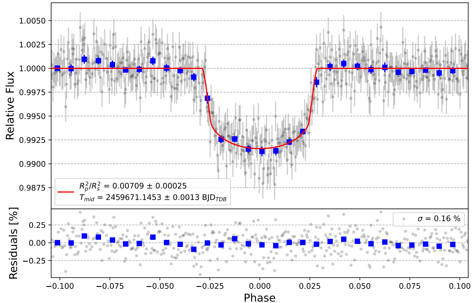
HAT-P-4 b
