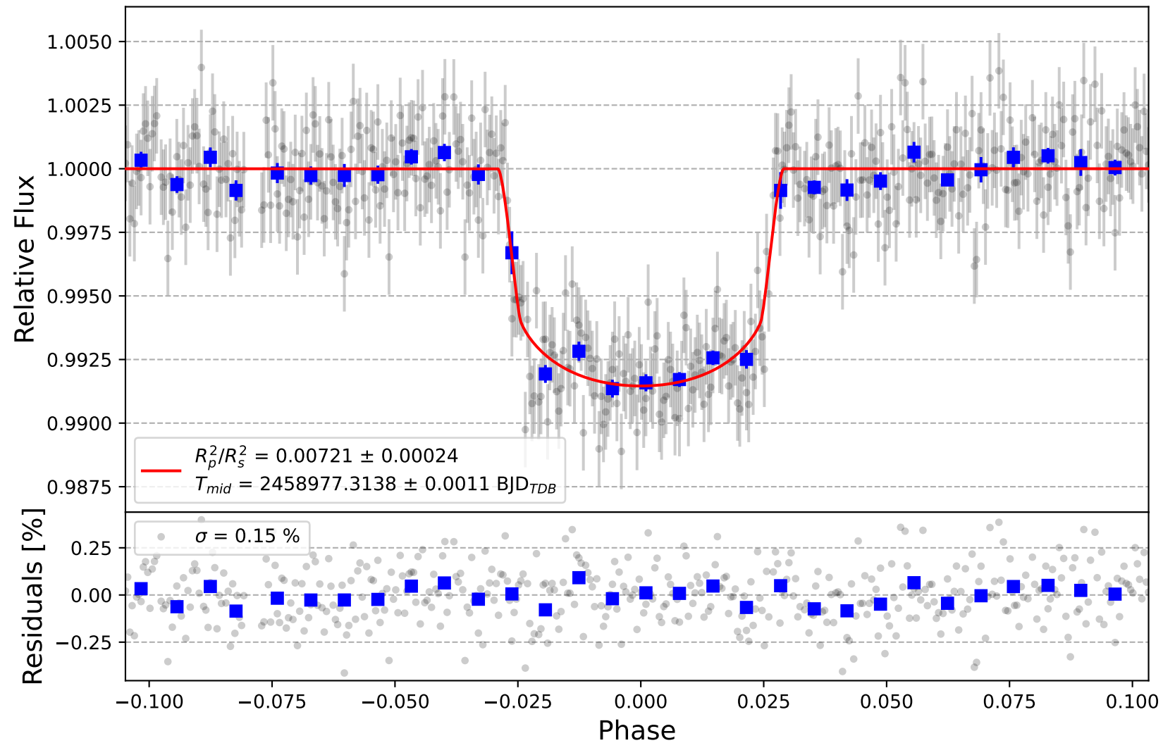
HAT-P-4 b
