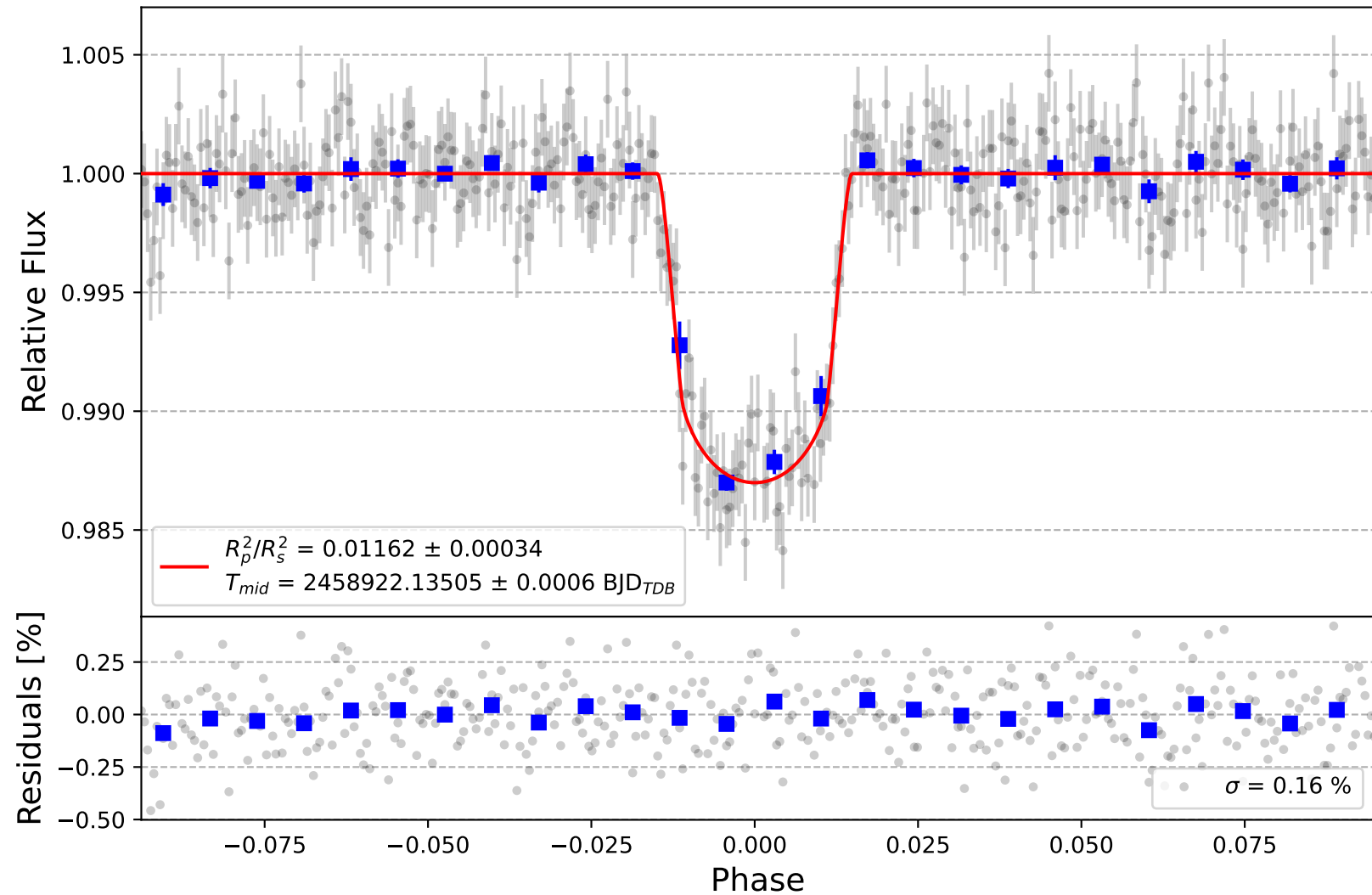
HAT-P-3 b
