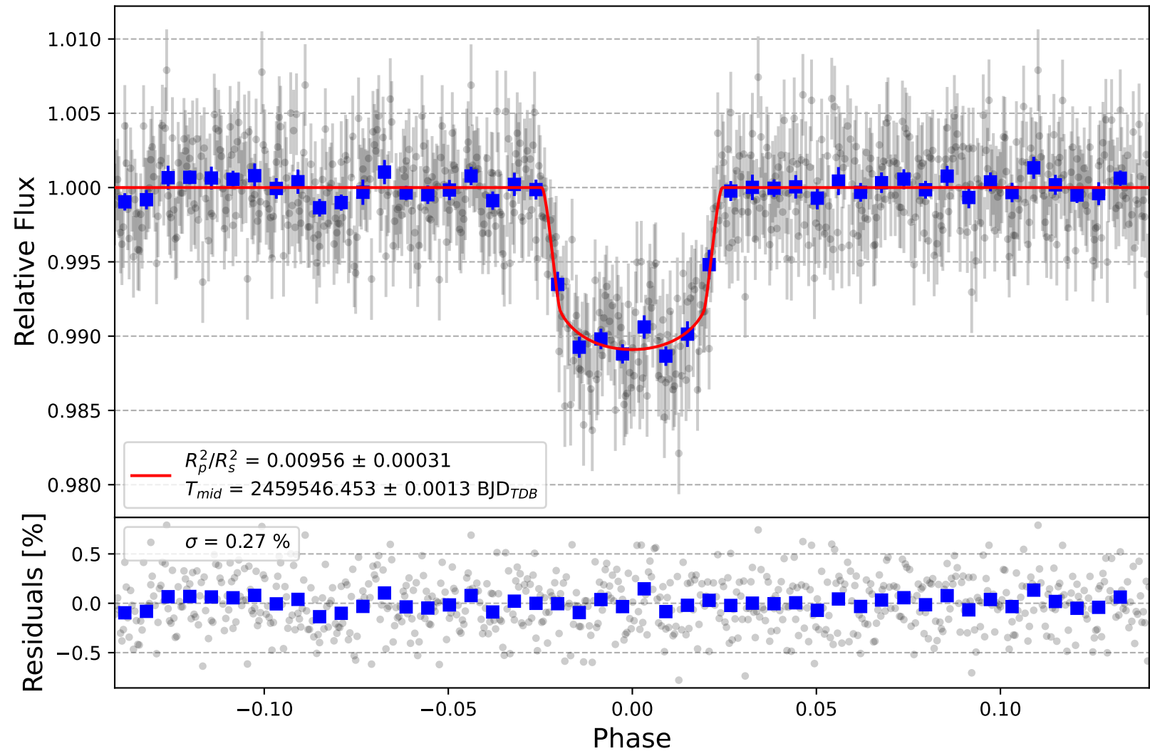
HAT-P-39 b
