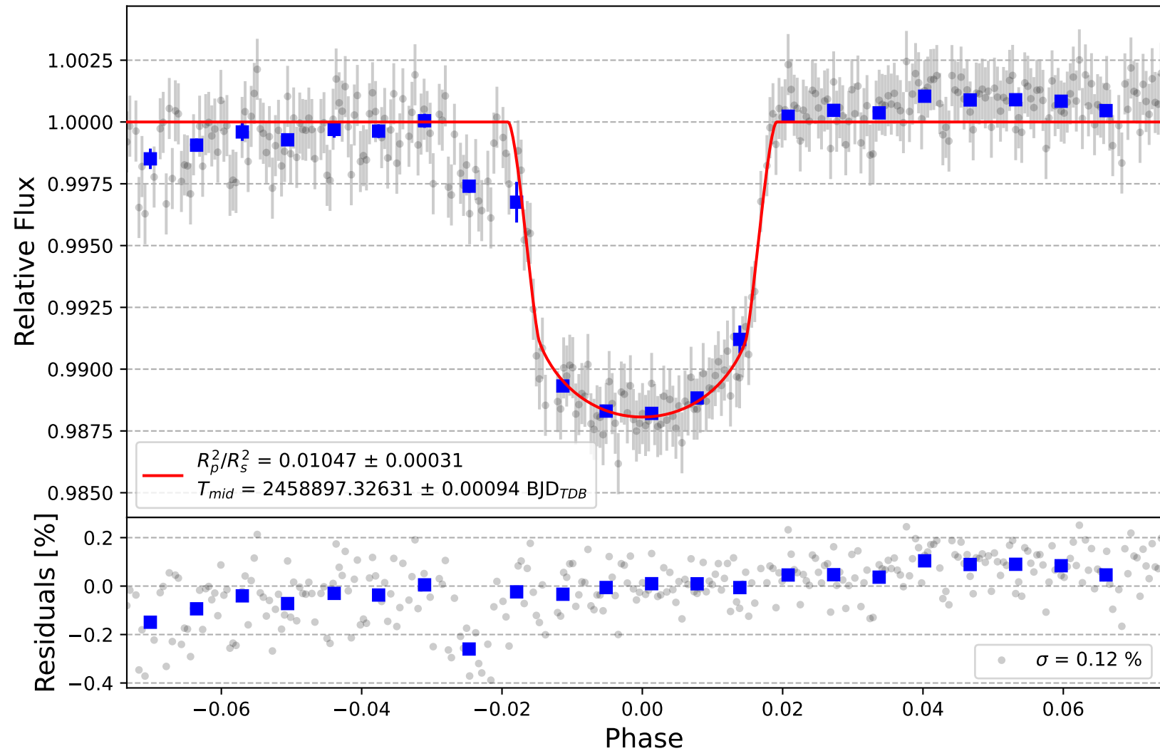
HAT-P-22 b
