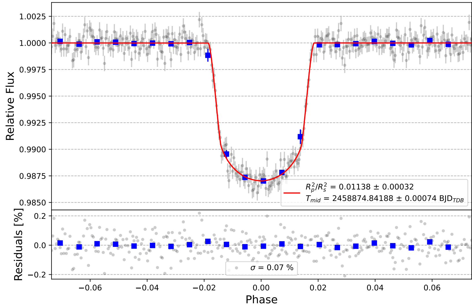
HAT-P-22 b
