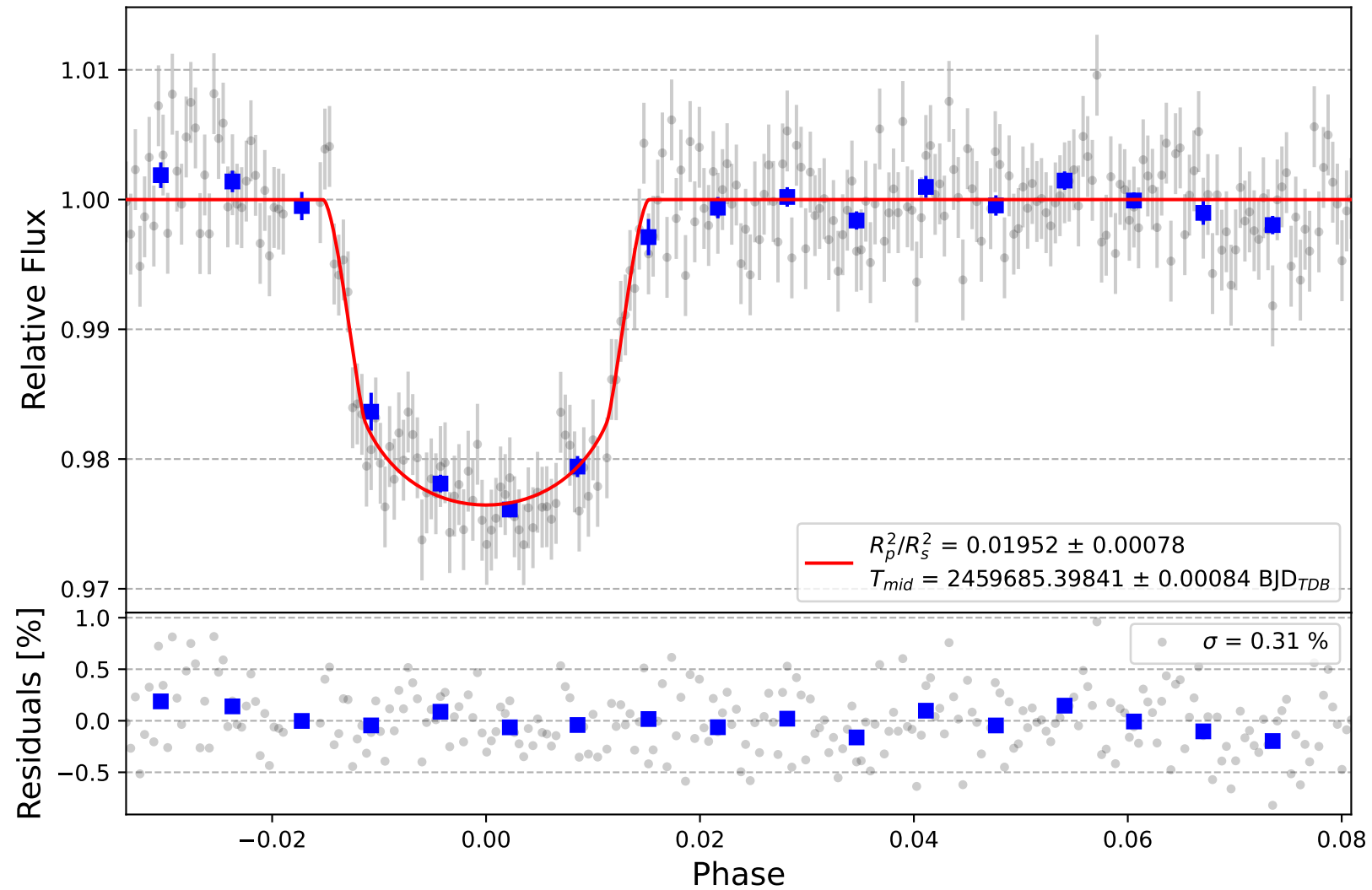
HAT-P-12 b
