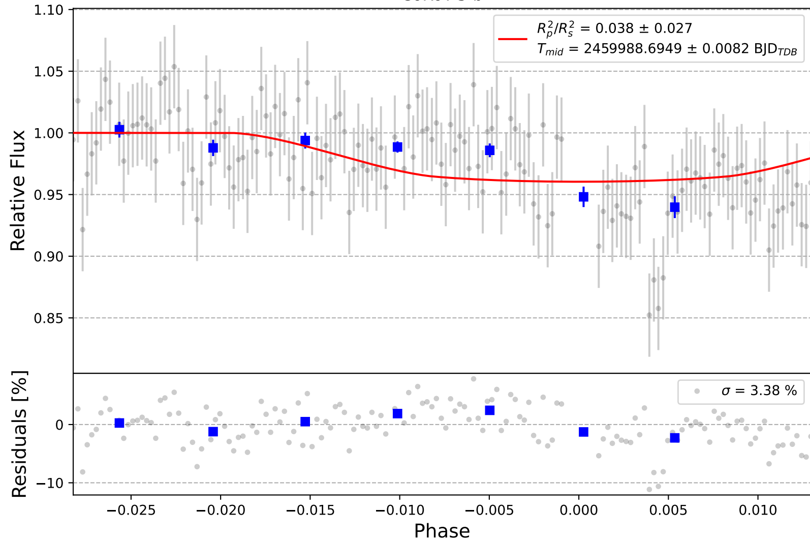
CoRoT-5 b
